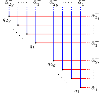
FIGURE 5. The bounded regions of the diagram (\hat{F}, \{\tilde{\alpha}_i^-\}, \{\tilde{\alpha}_i^+\})
