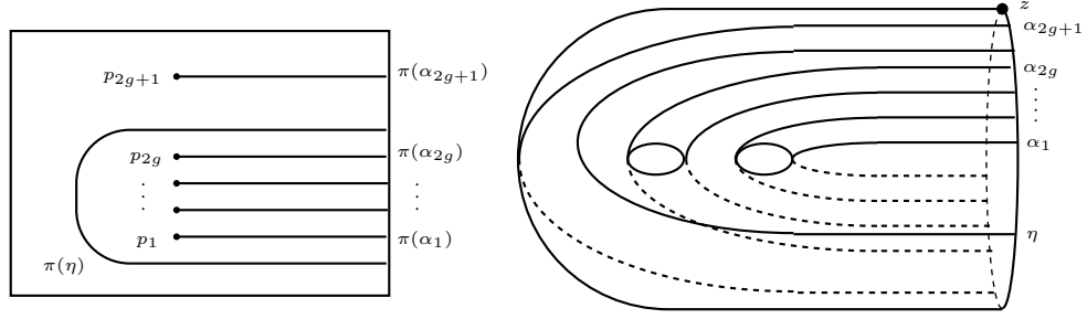
FIGURE 8. Isotoping \alpha_{2g+1} into \pi^{-1}(\{\text{Im } w < 0\})
