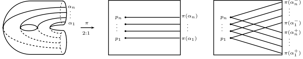
FIGURE 1. The arcs \alpha_j and \alpha_j^\pm
