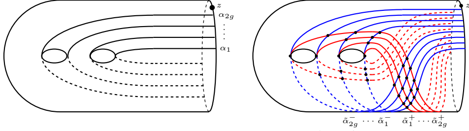
FIGURE 4. The arcs \alpha_j and \tilde{\alpha}_j^\pm on \hat{F}
