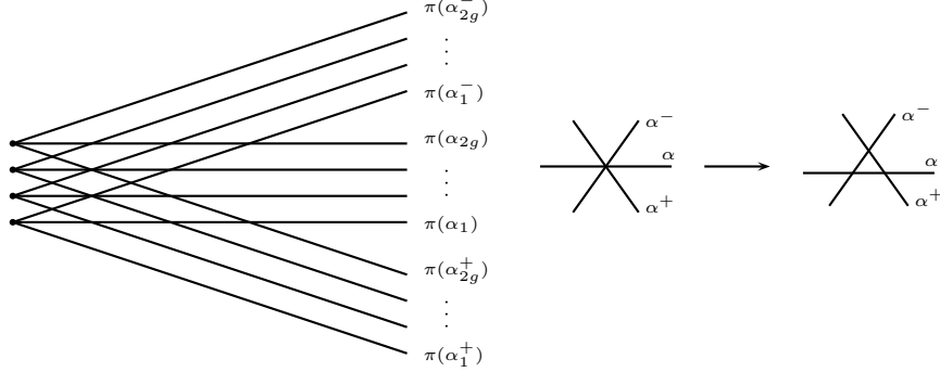
FIGURE 3. The projection of the triple diagram (F', \alpha_i^-, \alpha_i, \alpha_i^+)
