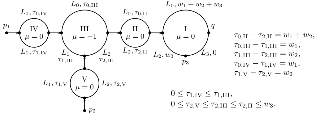
FIGURE 10. A rigid cascade contributing to m_3^\emptyset . The arrows indicate intersections that match via the flow \phi_{H_\rho} .
