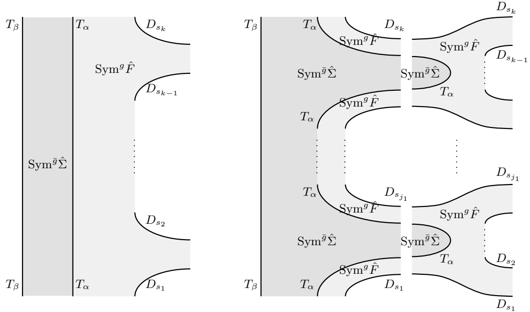
FIGURE 9. The \mathcal{A}(F, g) -module structure on \bigoplus CF^*(\bar{\Phi}_\alpha(T_\beta), D_s) (left) and the \Phi_\alpha(\mathcal{A}(F, g)) -module structure on \bigoplus CF^*(T_\beta, \Phi_\alpha(D_s)) (right)
