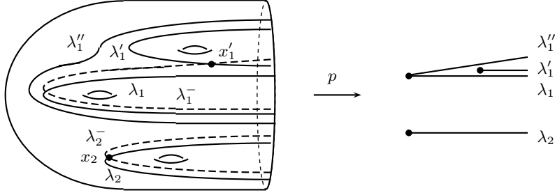
FIGURE 7. Sliding \lambda_1 along \lambda'_1 , and the covering p
