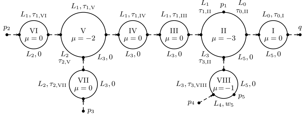
FIGURE 11. A rigid cascade contributing to m_5^{\{2,3,4\}} . The dotted lines indicate intersections that match via the maps \vartheta_w^{w'} from A.1(2).
