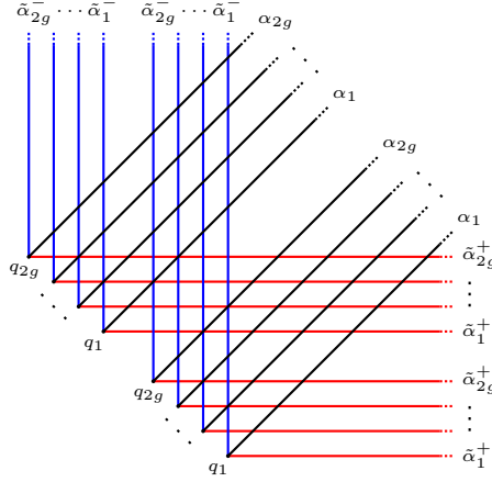
FIGURE 6. The bounded regions of the diagram (\hat{F}, \{\tilde{\alpha}_i^-\}, \{\alpha_i\}, \{\tilde{\alpha}_i^+\})
