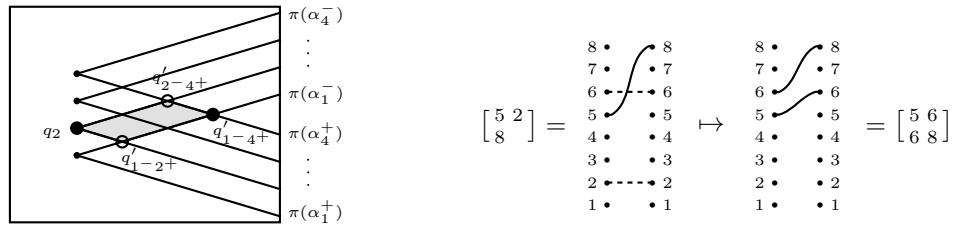
FIGURE 2. An empty rectangle and the corresponding differential.
