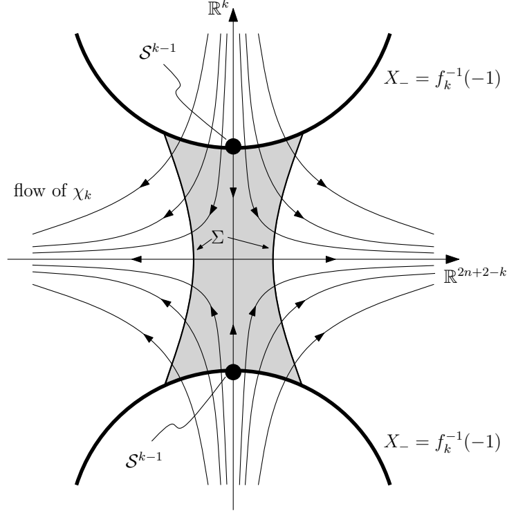
FIGURE 1. Weinstein handle H_k (shaded) and the flow of \chi_k transverse to \partial H_k .
