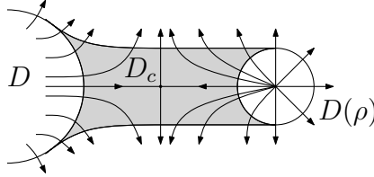
FIGURE 5. Constructing an exact symplectic structure on D' = D \cup D_c \cup D(\rho) .
