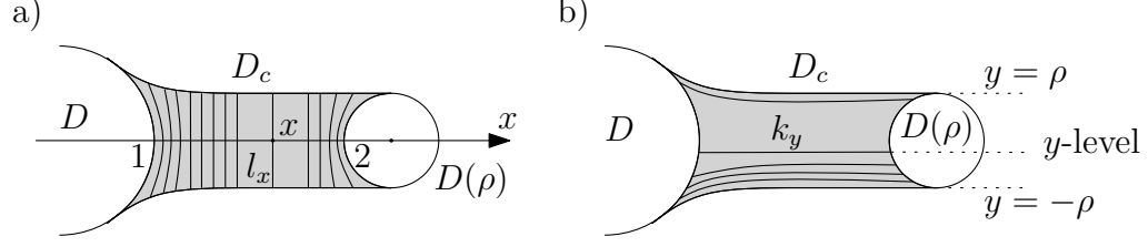
FIGURE 4. a) Vertical foliation \{l_x \mid x \in [1, 2]\} on D_c , b) Horizontal foliation \{k_y \mid y \in [-\rho, \rho]\} on D_c .
