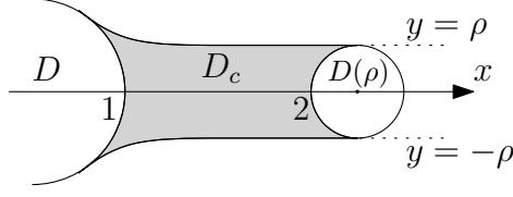
FIGURE 3. The disk D_c connecting D and D(\rho) .
