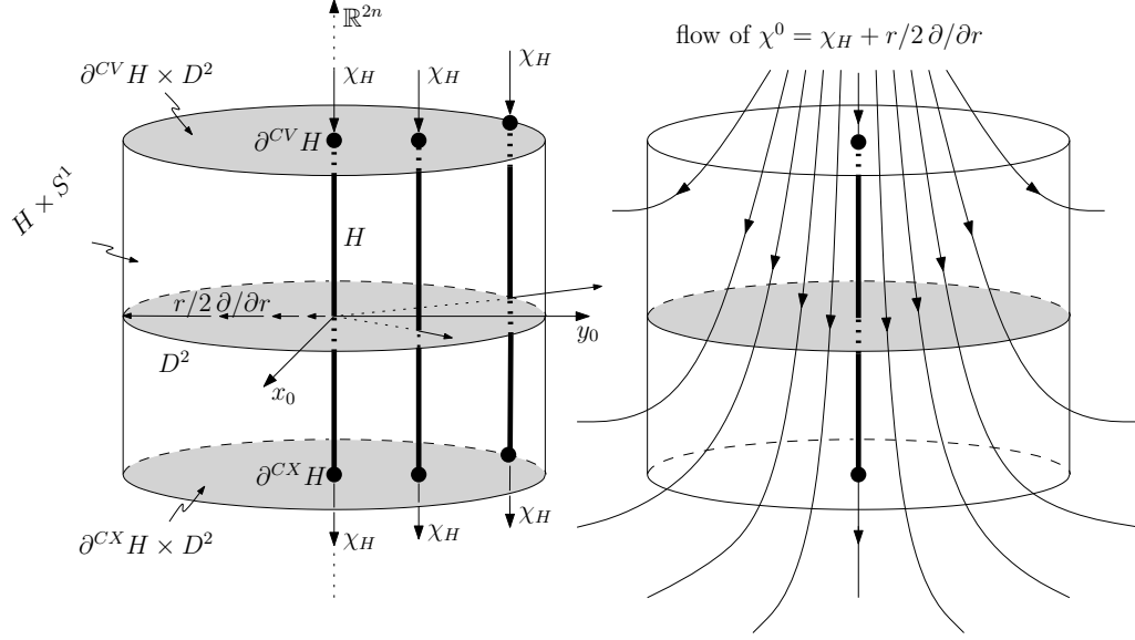
FIGURE 2. A schematic picture of the convex and concave parts of \partial H_n and the flow of \chi^0 = \chi_H + r/2 \partial/\partial r in \mathbb{R}^{2n} \times \mathbb{R}^2 .
